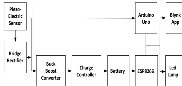
Figure 8: Block Diagram
